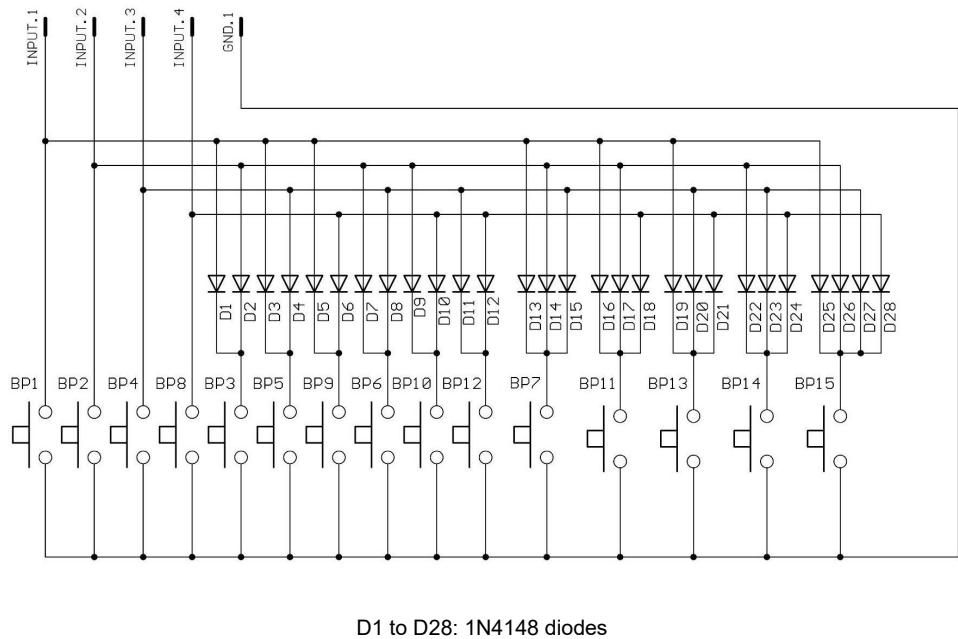
15 push-buttons mapped to 4 inputs
