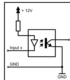
Figure 3: Internal schematic of a player input
