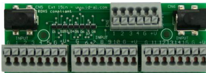
Figure 2: Optional extension board
