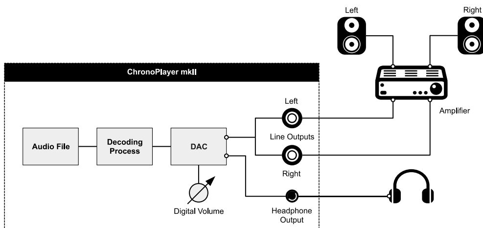
Figure 7: Audio diagram of the ChronoPlayer mkII
